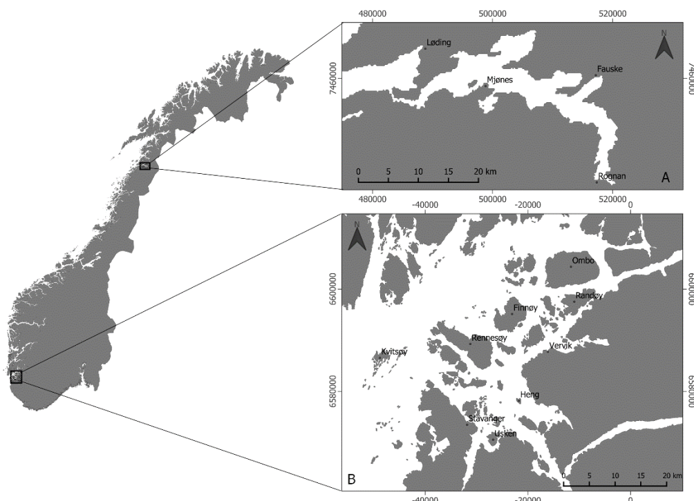
Figure 4.18. Selected focus areas. A – Skjerstadfjorden, inner Saltfjorden and associated waterbodies and B – fjordsystems north of Stavanger.
