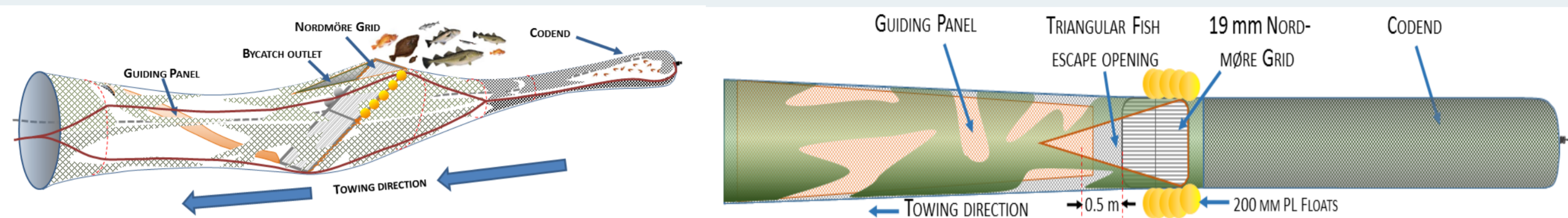
The working principle of a Nordmøre grid bycatch excluder system and design details
