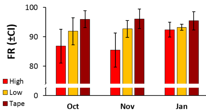
Fig. 12: Fouling resistance of 4 tested surfaces during a 10 months trial, with a detailed depiction of the three antifouling films in the last months of the trial.
