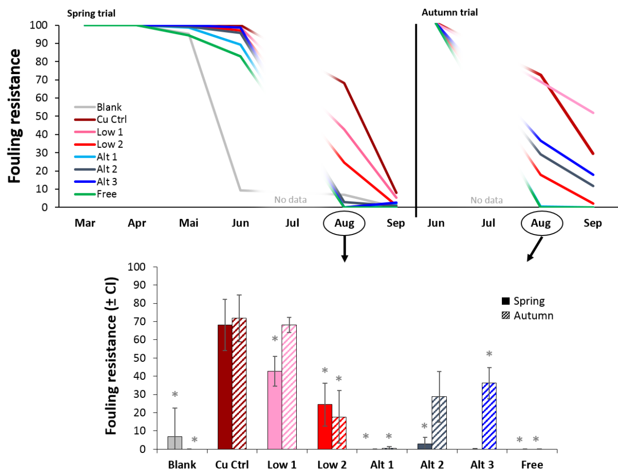
Fig. 5: Fouling Resistance of 8 different coatings of net samples in the spring (6 months duration) and an autumn (3 months duration) trial, including a detailed depiction of the situation in August of both trials. Coatings with significantly lower FR values than the copper control are indicated by an asterisk
