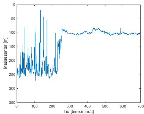
Figur 12: Estimert massesenter.
