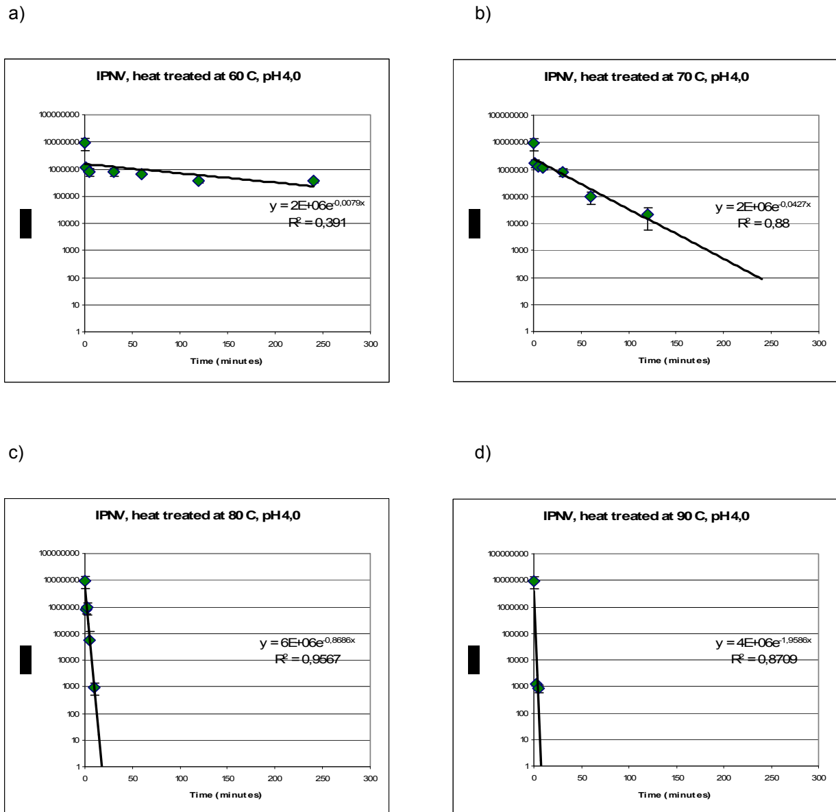
Figure 8 Inactivation curves for IPNV in artificial medium (pH 4,0) during heat treatment at 60,0 °C (a), 70,0 °C (b), 80,0 °C (c) and 90,0 °C (d). The straight lines are regression exponential curves. Each data point is the average of two parallel analyses. Vertical bars represent the standard deviation.
